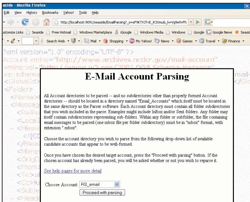
The Web User Interface of the CERP parser that outputs an email collection into an XML file of the account following the Email Account XML Schema. The parser code will be released soon.
